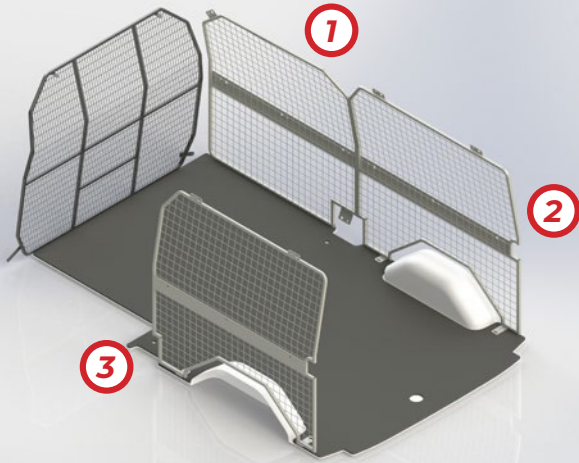
Mesh Wall Panelling - all options (Cargo Barrier sold Separately)
